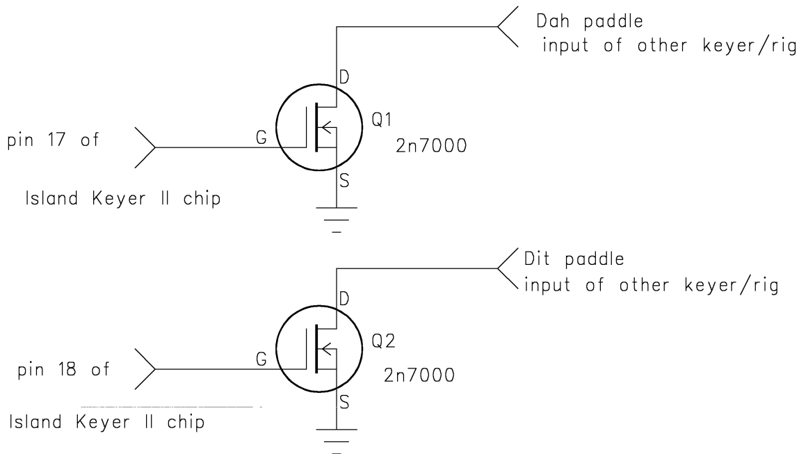
Island Keyer II paddle output circuit (output from the IK2 to another keyer paddle inputs)
