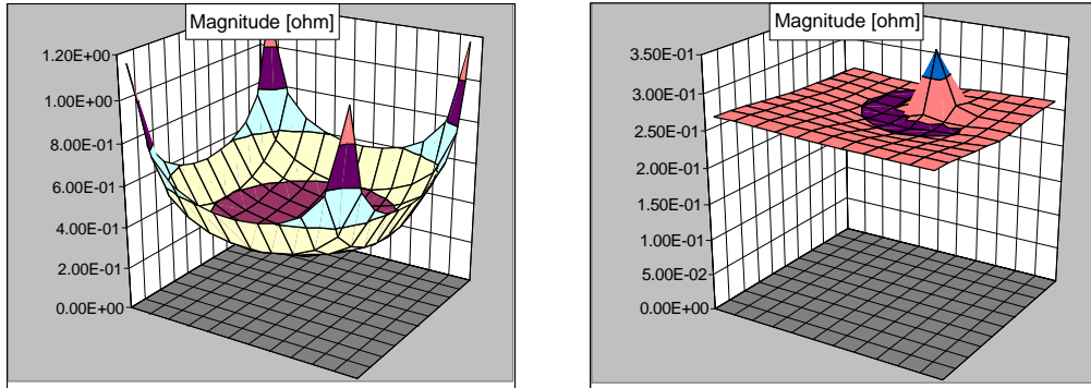
Magnitude of self-impedance (on the left) and transfer-impedance (on the right) plots at 100MHz. The transfer impedance is shown from 3 inches and 4 inches away from the corner, where the peak of the impedance profile occurs.
