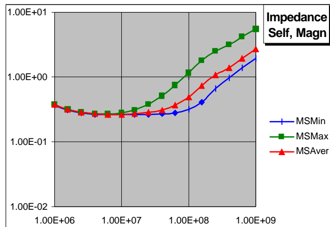
Minimum, average and maximum values of the simulated self-impedance magnitudes (in ohms) over the planes at various frequencies (in Hertz).]
