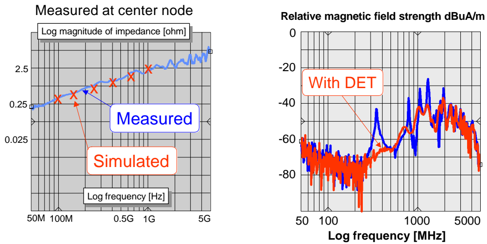
On the left, comparison of measured and simulated self-impedance magnitude values of DUT at the center of the planes. On the right, comparison of measured edge radiation with and without edge termination.
