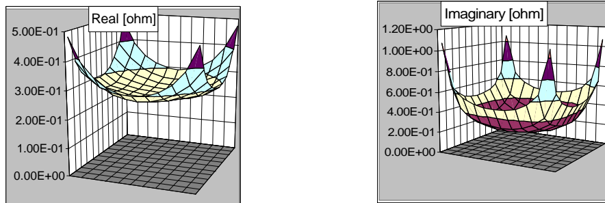
Simulated real and imaginary part of the self-impedance profile at 100MHz. The impedances are plotted at every inch of the grid.
